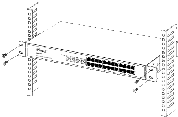
Figure 2-2 Fasten the Switch in the rack
